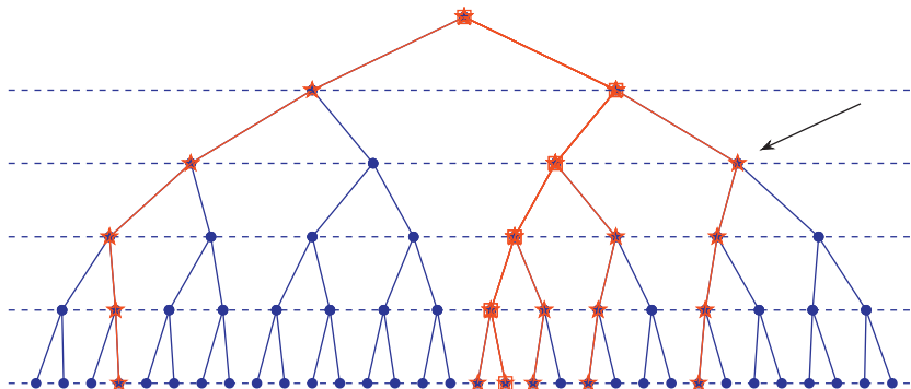
Fig. 1. Tree-search algorithm for a system with N=5 and K=5 antennas and a given \mathbf{H} . The transmitted bit vector is \mathbf{x} = (1, -1, -1, -1, 1)^T . Paths with stars are provided by the dominance conditions alone, while the path with square nodes is the ML solution.
