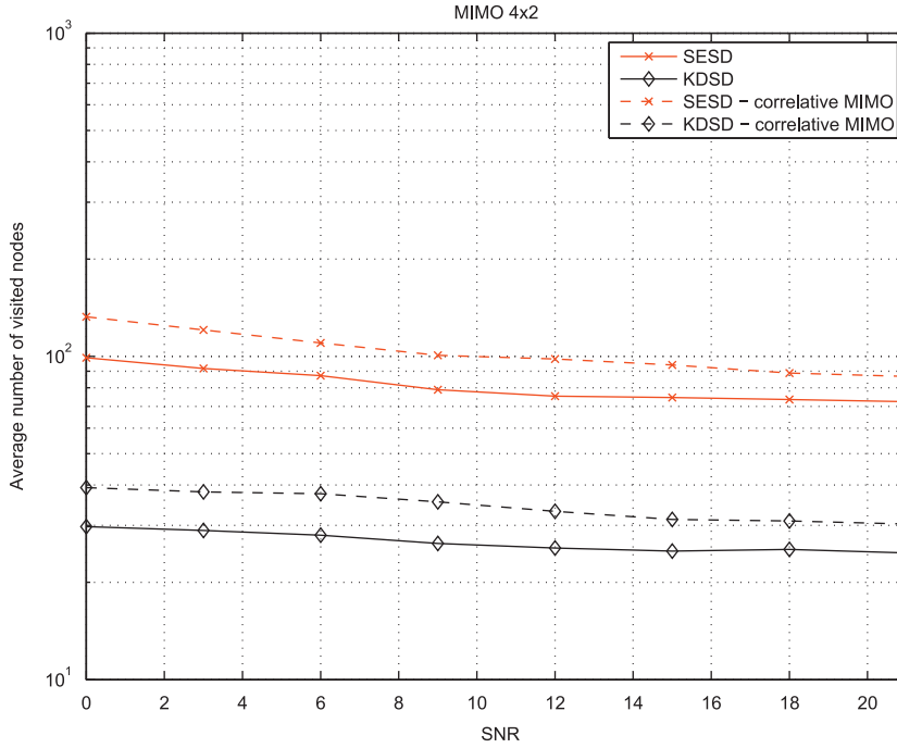
Fig. 4. Average number of visited nodes as a function of average signal-to-noise ratio. 16-QAM system with K=2 , N=4 .
