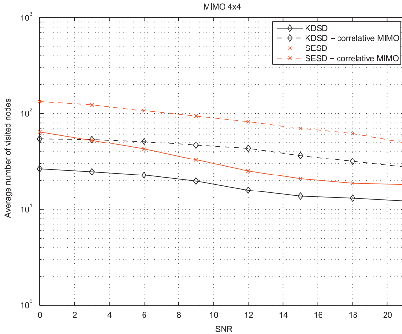
Fig. 3. Average number of visited nodes as a function of average signal-to-noise ratio. 4-QAM system with K=4 , N=4 .
