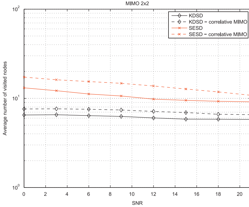
Fig. 2. Average number of visited nodes as a function of average signal-to-noise ratio. 4-QAM system with K=2 , N=2 .
